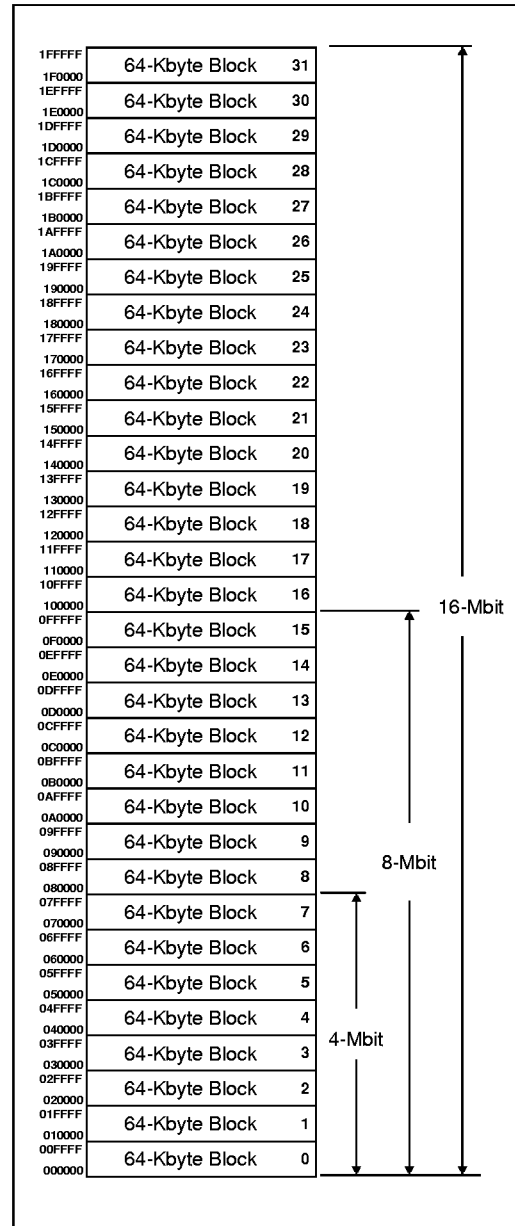
Figure 4. Memory Map
