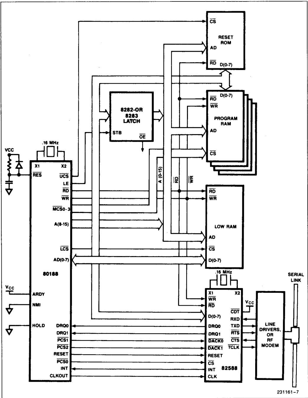
Figure 10. 80188 Based System
