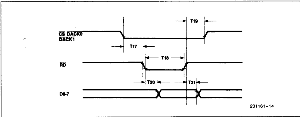
Read Timing
