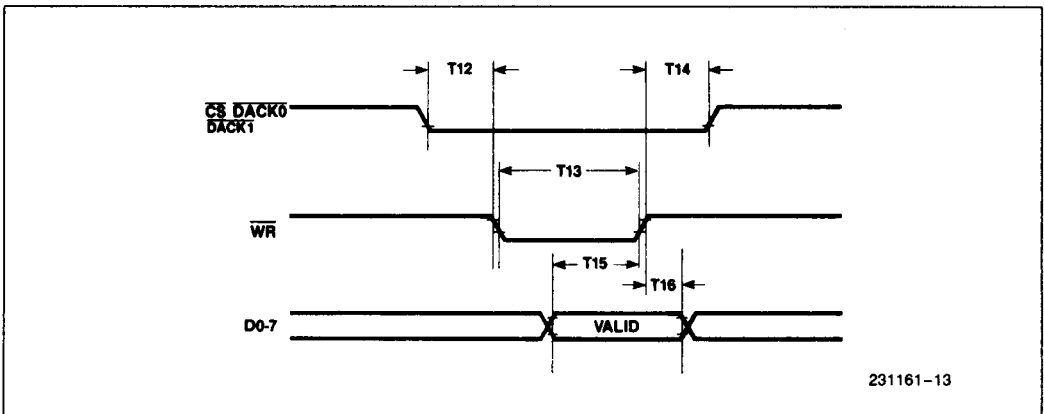
Write Timing
