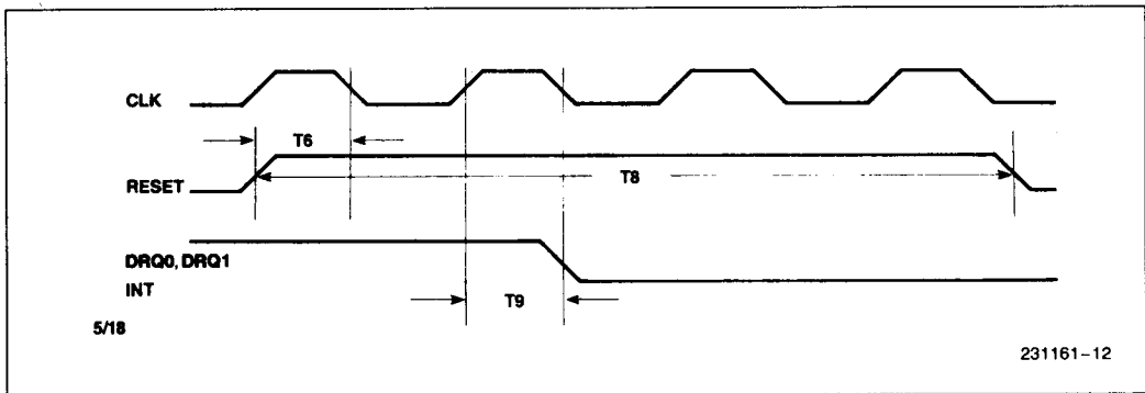
Reset Timing
