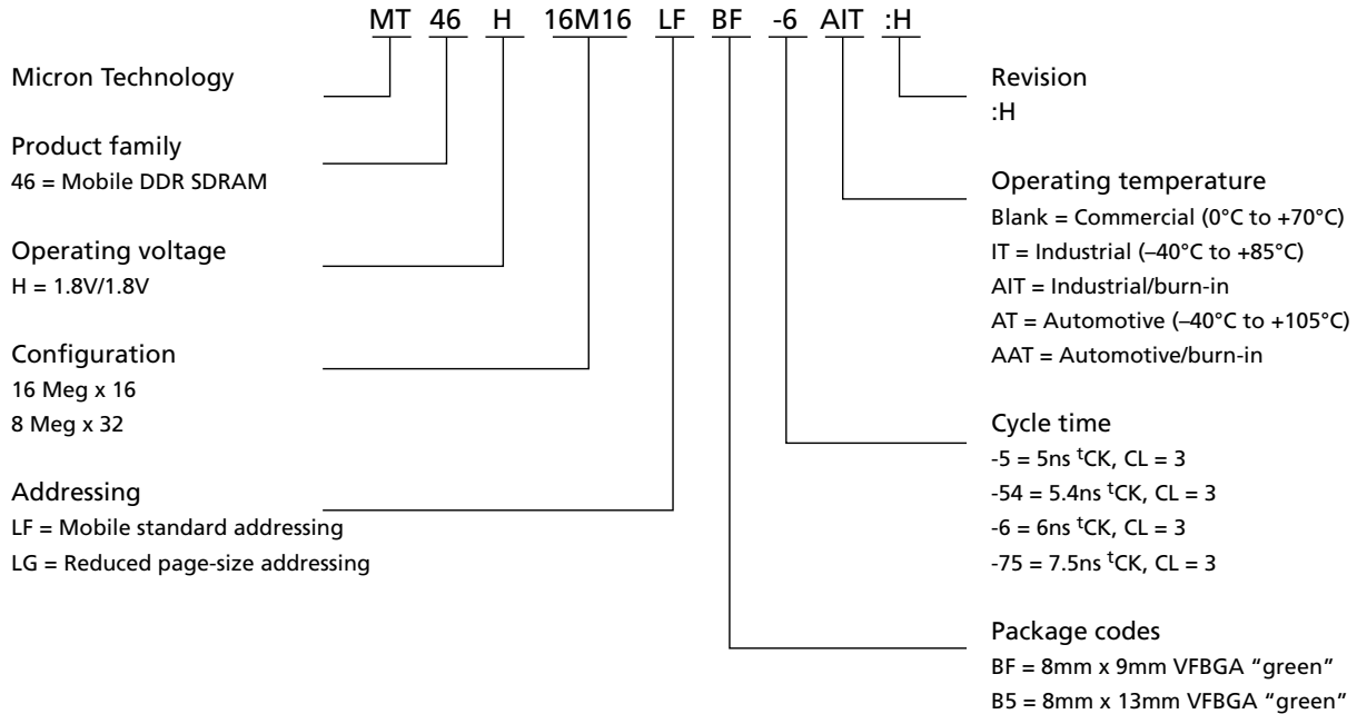
Figure 1: 256Mb Mobile LPDDR Part Numbering
