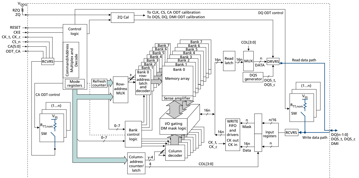
Figure 5: Functional Block Diagram
