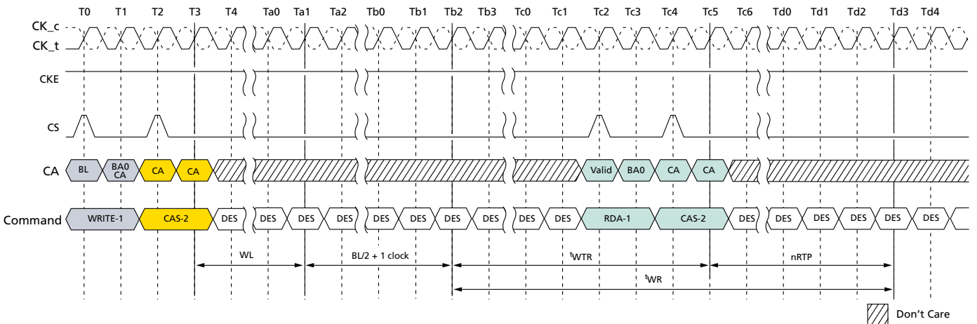
Figure 66: Delay Time From WRITE-to-READ with Auto Precharge
