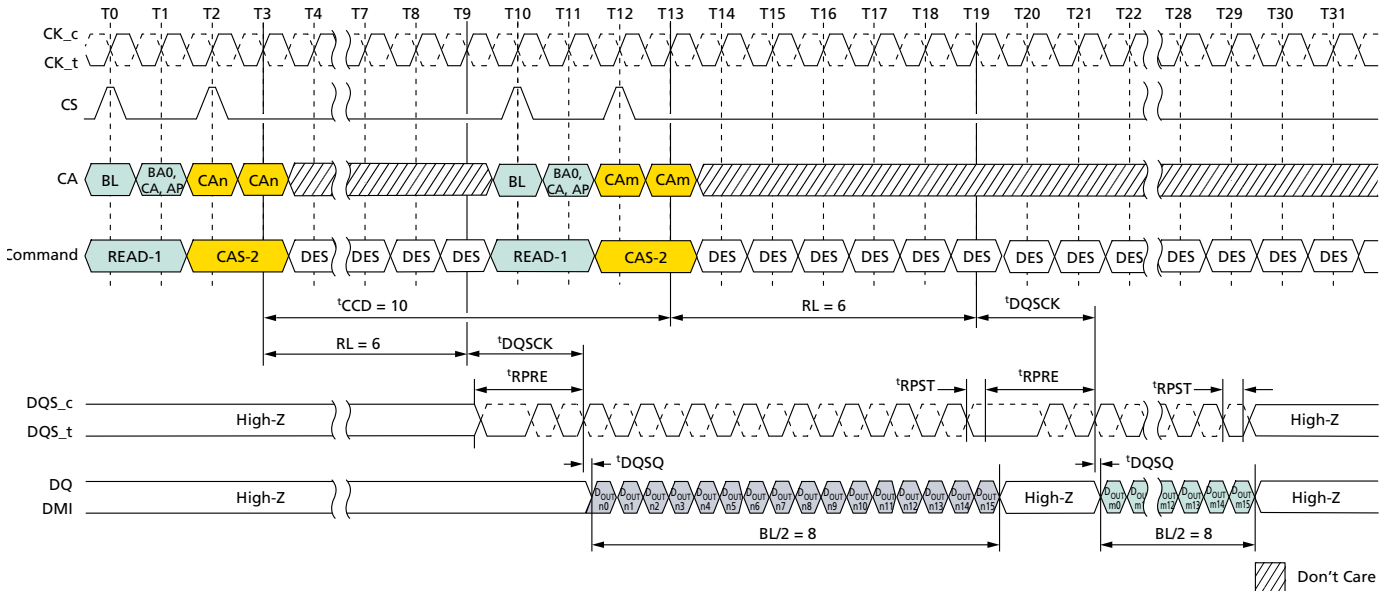
Figure 42: Consecutive READ: t_{CCD} = MIN + 2 , Preamble = Toggle, 0.5nCK Postamble
