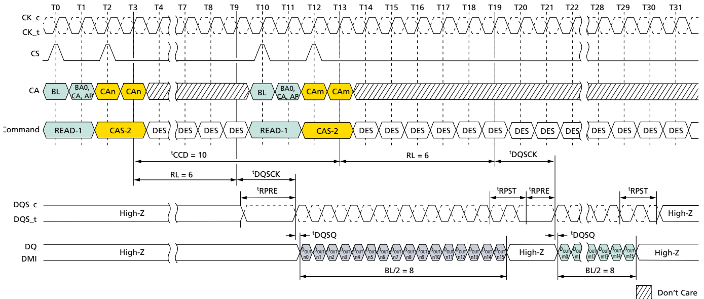
Figure 43: Consecutive READ: t_{CCD} = MIN + 2 , Preamble = Static, 1.5nCK Postamble
