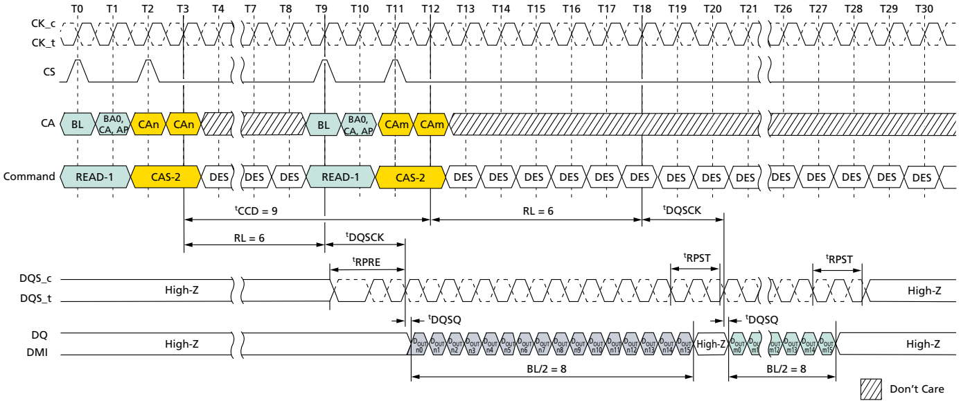
Figure 37: Seamless READ: t_{CCD} = MIN + 1 , Preamble = Toggle, 1.5nCK Postamble
