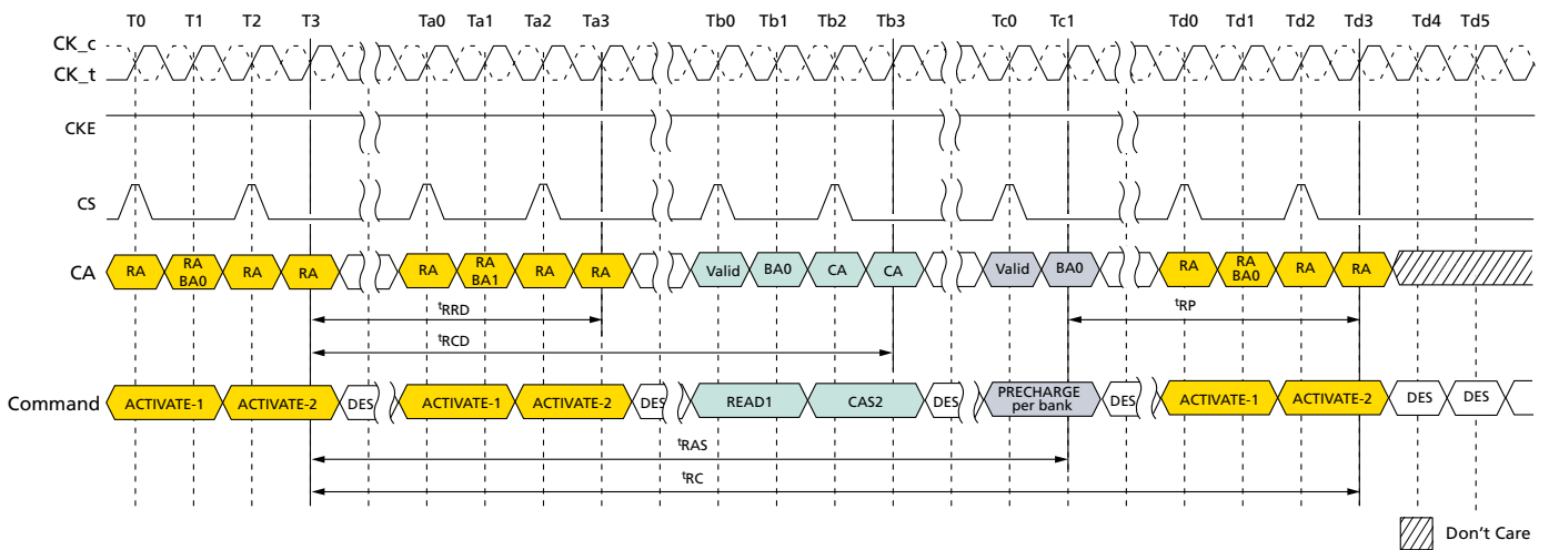
Figure 9: ACTIVATE Command
