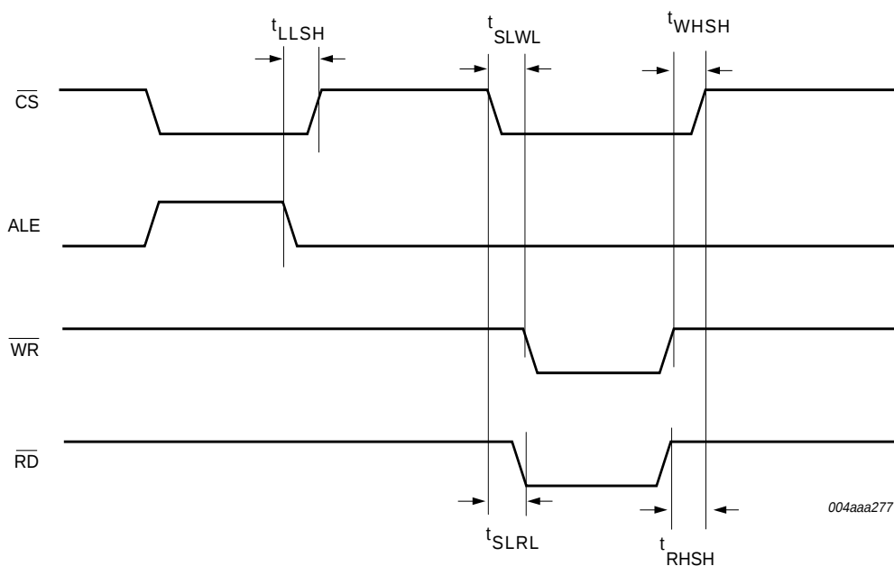
Fig 16. Set-up and hold time.
