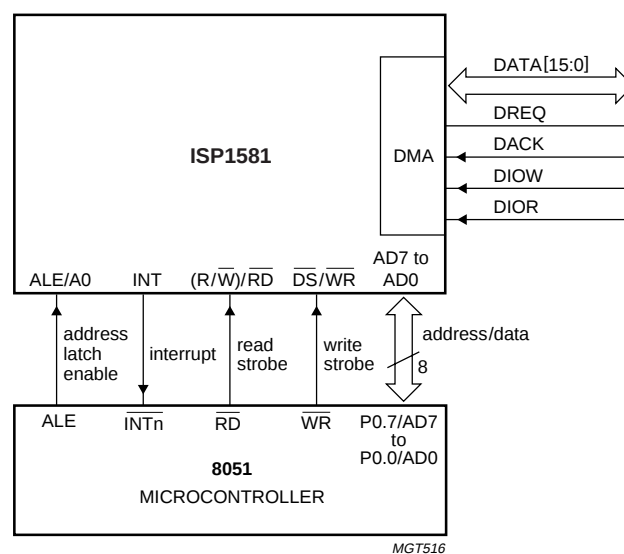
Fig 39. Typical interface connections for Split Bus mode (slave mode).
