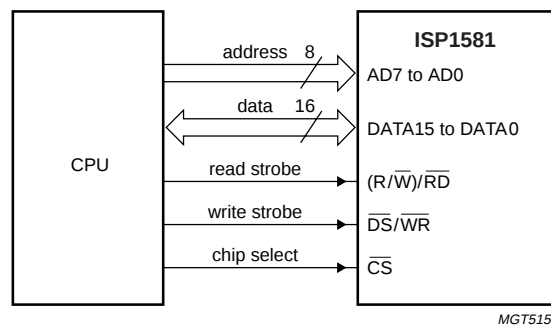
Fig 38. Typical interface connections for Generic Processor mode.
