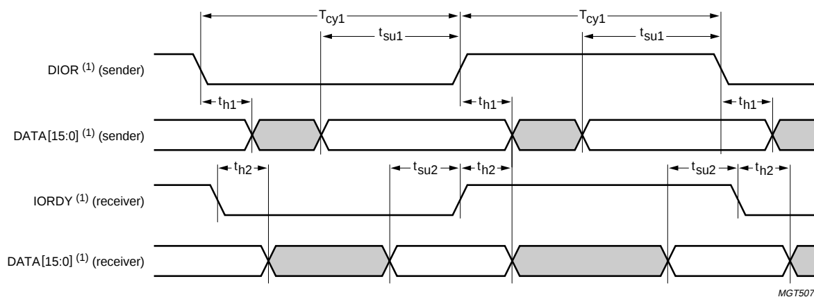
Fig 30. UDMA timing: sustained synchronous burst.
