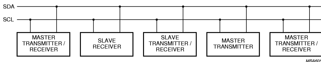
Fig.6 System configuration.
