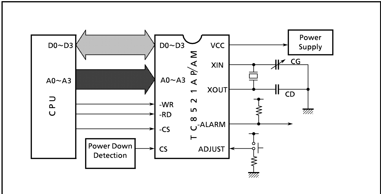
FIG.3.2 SYSTEM CONFIGURATION
