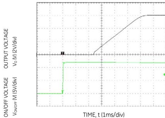
Figure 41. Typical Start-up Using On/Off Voltage ( I_o = I_{o,max} ).
