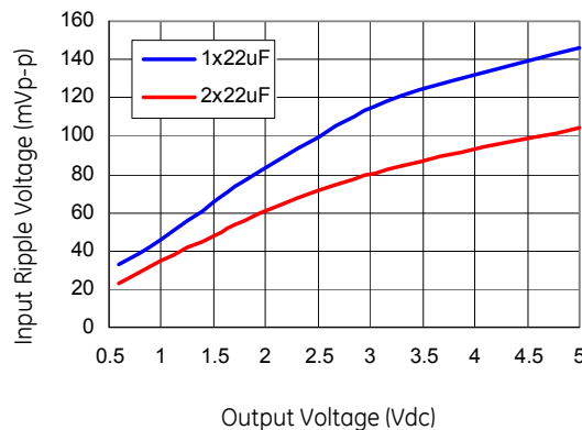
Figure 46. Input ripple voltage for various output voltages with 1x22 μF or 2x22 μF ceramic capacitors at the input (6A load). Input voltage is 12V.
