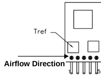
Figure 54. T_{ref} Temperature measurement location.
