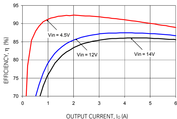
Figure 73. Converter Efficiency versus Output Current.
