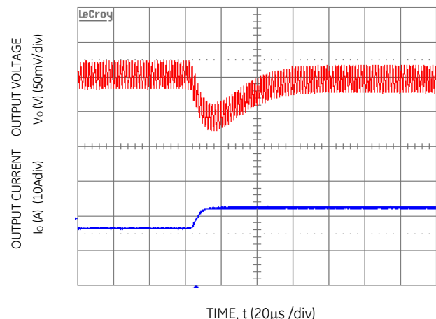
Figure 28. Transient Response to Dynamic Load Change from 50% to 100% at 12Vin, C_{out}=1\times 47\mu\text{F}+1\times 330\mu\text{F} , C_{Tune}=2700\text{pF} & R_{Tune}=330\text{ohms}
