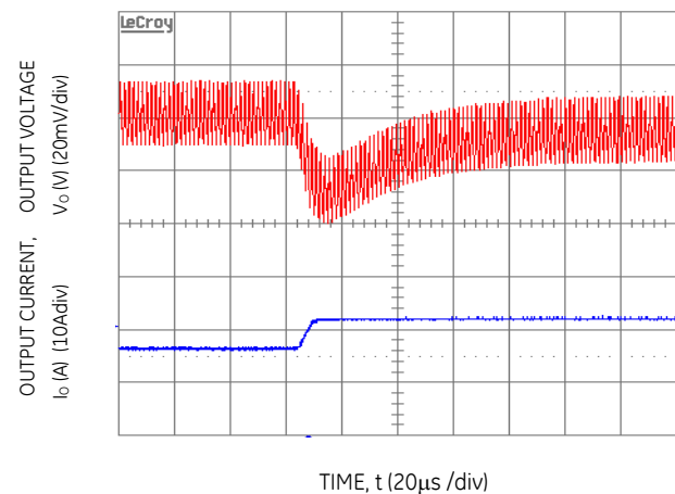
Figure 16. Transient Response to Dynamic Load Change from 50% to 100% at 12Vin, C_{out}=1\times 47\mu\text{F}+2\times 330\mu\text{F} , C_{Tune}=5600\text{pF} & R_{Tune}=270\text{ohms}
