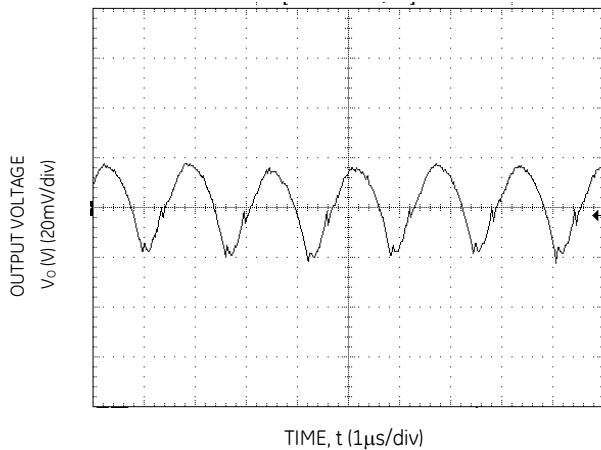
Figure 21. Typical output ripple and noise (C o =22μF ceramic, V IN = 12V, I o = I o,max ).
