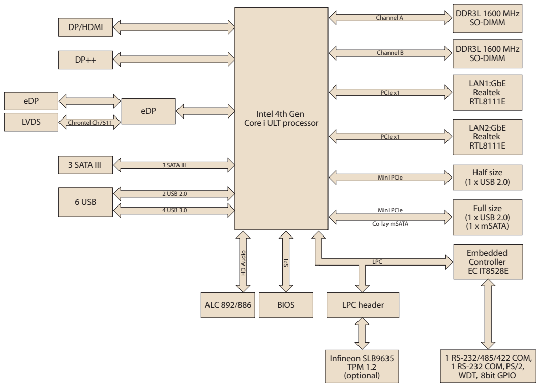
Figure 1.2 AIMB-230 Board Diagram
