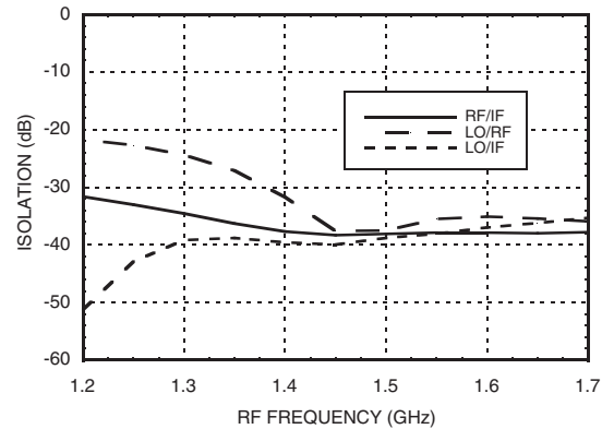
Isolation [2]
