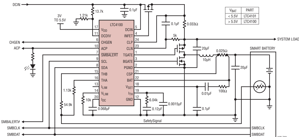
Figure 1. 4A Smart Battery Charger
