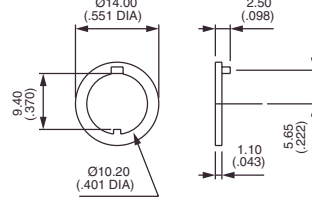
LOCKING RING
