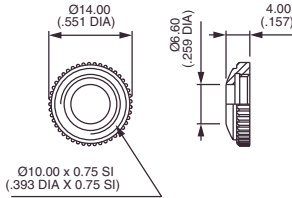
KNURLED CAP NUT (std for 10600)
