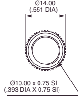
KNURLED NUT (std for 10400)
