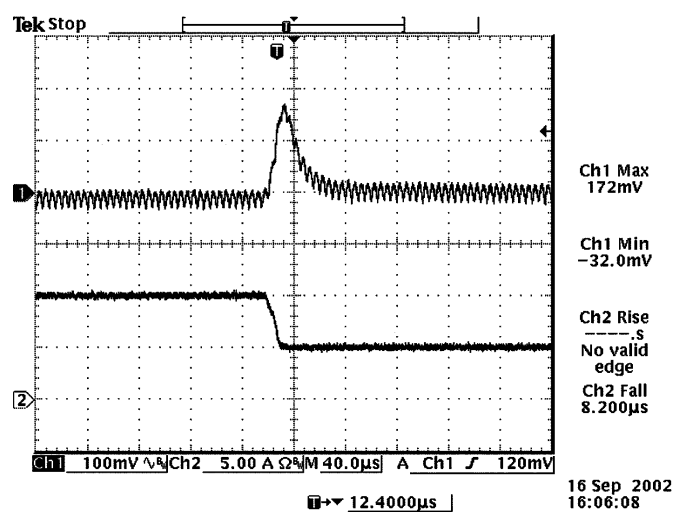
V_{out}=2.0V 100% to 50% load transients at 12V input and T_a=25^\circ C
