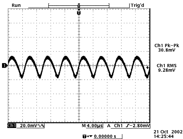
Ripple and noise at full load and 12Vdc input, 1.8Vdc output, full load with an external 22µF tantalum capacitor and Ta=25° C
