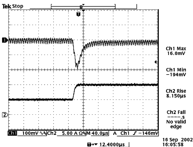
V_{out}=2.0V 50% to 100% load transients at 12V input and T_a=25^\circ C
