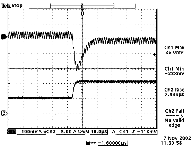
Vout=3.3V 50% to 100% load transients at 12V input and Ta=25° C
