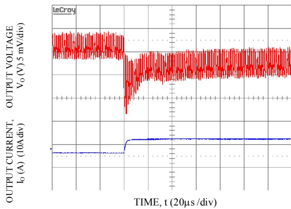
Transient Response to Dynamic Load Change from 50% to 100% at 12Vin, Cout-3x47uF+6x330uF, CTune-47nF, RTune-180ohms. Vo=0.6V
