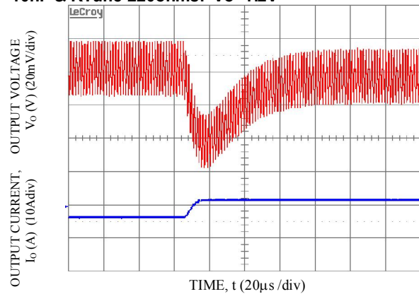
Transient Response to Dynamic Load Change from 50% to 100% at 12Vin, Cout-1x47uF+1x330uF, CTune-3300pF & RTune-270ohms. Vo=2.5V
