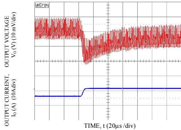
Transient Response to Dynamic Load Change from 50% to 100% at 12Vin, Cout-1x47uF+3x330uF, CTune-10nF & RTune-220ohms. Vo=1.2V
