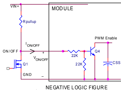
NEGATIVE LOGIC FIGURE Circuit configuration for using negative On/Off logic.
