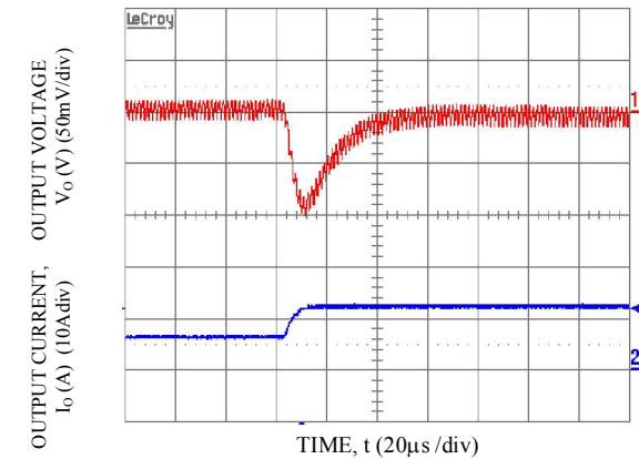
Transient Response to Dynamic Load Change from 50% to 100% at 12Vin, Cout-5x47uF, CTune-1500pF & RTune-330ohms. Vo=5.0V
