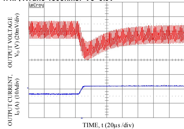
Transient Response to Dynamic Load Change from 50% to 100% at 12Vin, Cout-1x47uF+2x330uF, CTune-5600pF & RTune-270ohms. Vo=1.8V
