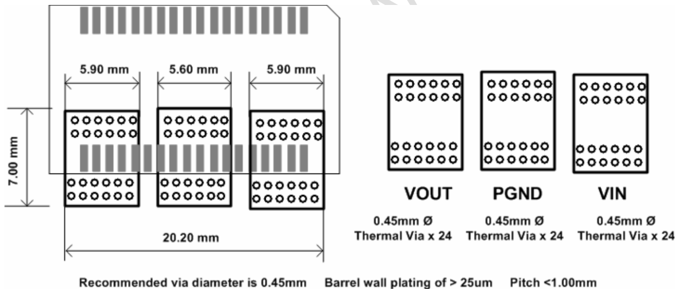
Figure 25. Recommended PCB Layout for Multilayer PCBs
