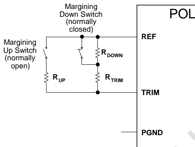
Figure 19. Margining Configuration
