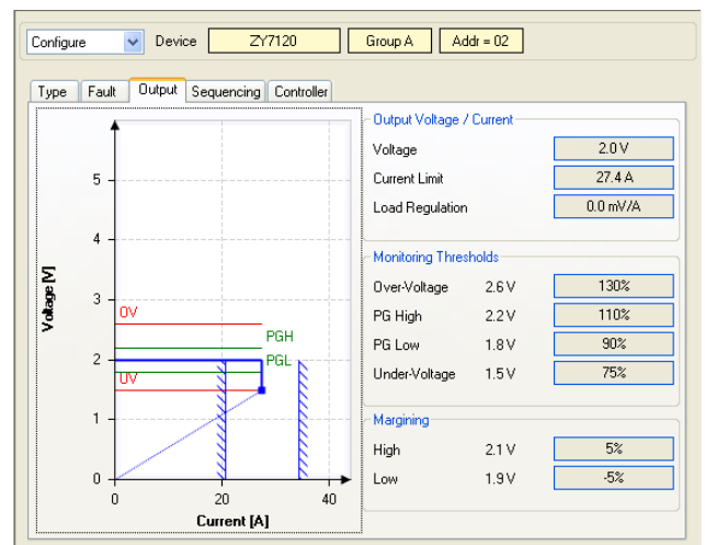
Figure 27. POL Configure Output Window
