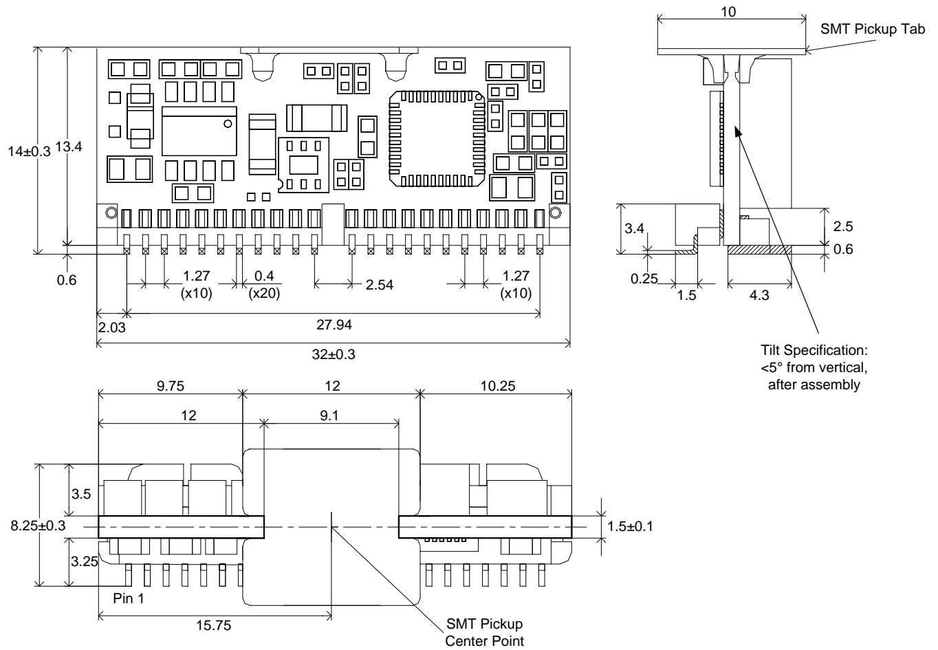
Figure 57. Mechanical Drawing
