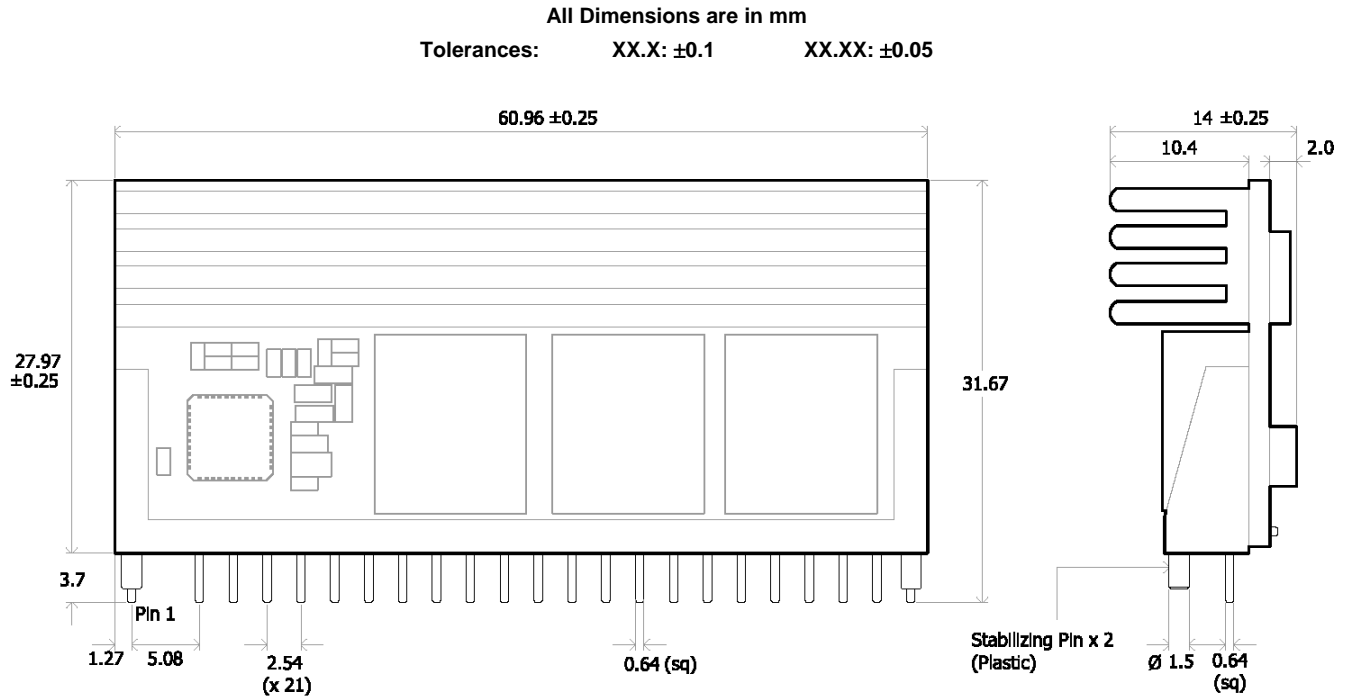
Figure 48. Mechanical Drawing
