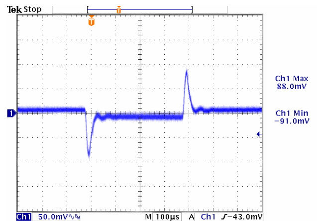
Figure 13. Vin=12V, Vout=1.8V
