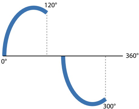
Trailing Edge Dimmer at 60°
