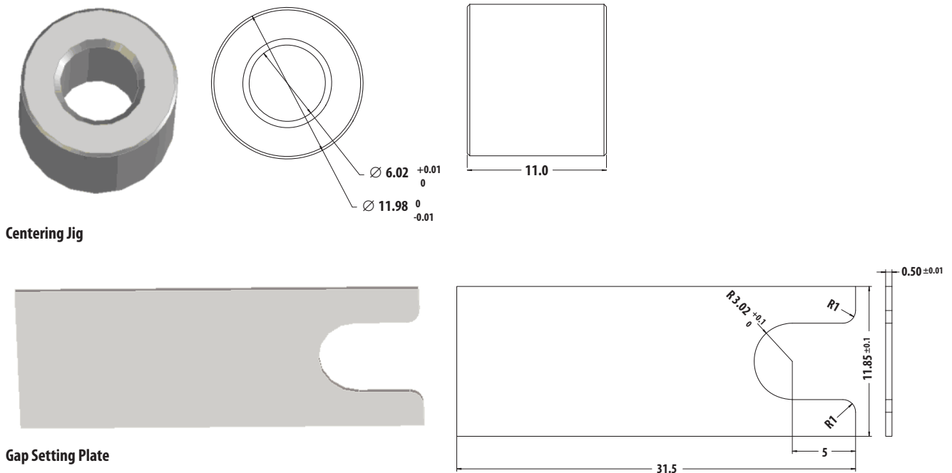
Figure 6. Alignment tool set and recommended dimensions
