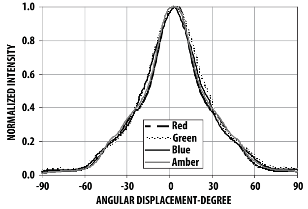
Figure 11b. Radiation Pattern for Minor Axis
