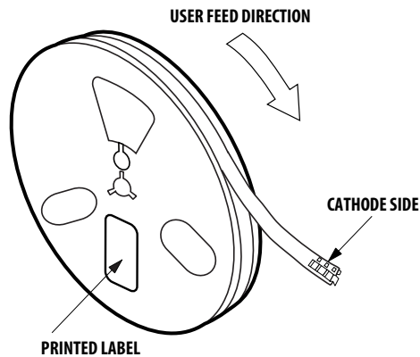
Figure 11. Reeling orientation.
