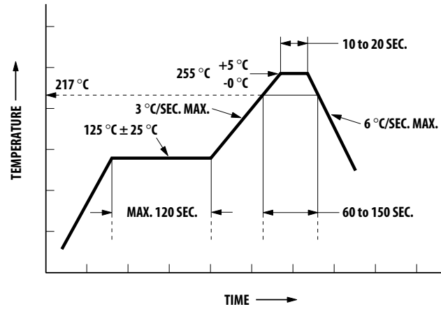
* THE TIME FROM 25 °C TO PEAK TEMPERATURE = 6 MINUTES MAX. Figure 6b. Recommended Pb-free reflow soldering profile.
