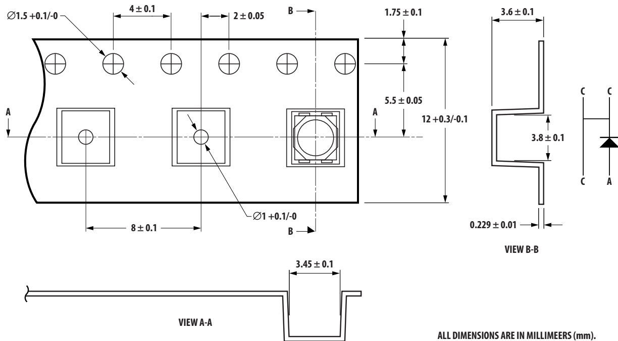
Figure 10. Tape dimensions.
