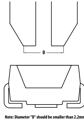
Figure 11. Recommended Pick and Place Nozzle Size
