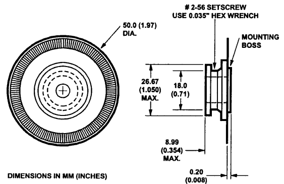
Figure 5. HEDS-6100 Codewheel.
