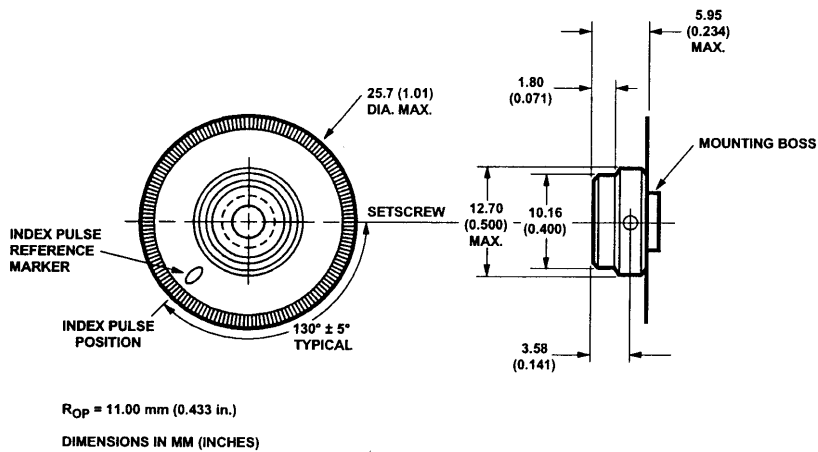
Figure 6. HEDS-5140 Codewheel Used with HEDS-9140.
