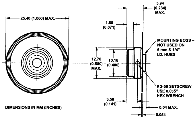
Figure 4. HEDS-5120 Codewheel.
