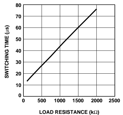
Figure 4. Switching characteristics.
