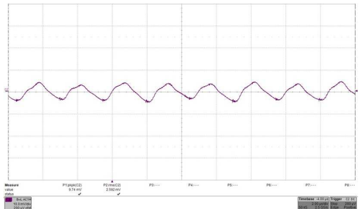
Fig. 30: Input reflected ripple current, i_c , measured at input terminals at full rated load current. Refer to Fig. 2 for test setup. RMS input ripple current i_c = 2.6 * 0.5A = 1.3A_{rms} .
