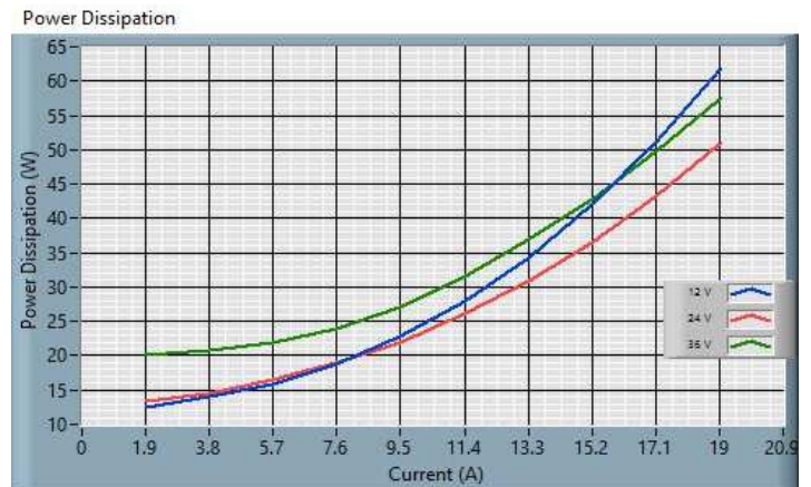
Fig. 14: 24S53.19FXP (ROHS) Power Dissipation
