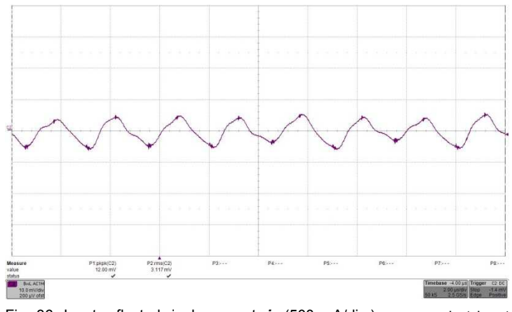
Fig. 36: Input reflected ripple current, i_c (500 mA/div.), measured at input terminals at full rated load current. Refer to Fig. 2 for test setup. RMS input ripple current i_c = 3.12 \cdot 0.5A = 1.56A_{rms} .
