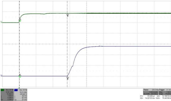
Fig. 25: Turn-on by ON/OFF transient ( V_{in} applied) at full rated load current (resistive). Top Trace (C1): ON/OFF signal, Bottom Trace (C4): Output voltage.
