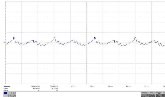
Fig. 41: Output voltage ripple at full rated load current.
