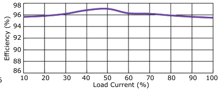
VX07815-500 Efficiency Curve Positive Output, Efficiency vs. Load Current (at Vin nominal)
