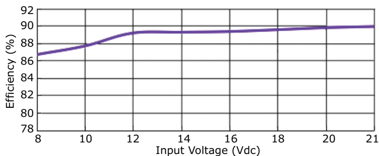
VX07815-500 Efficiency Curve Negative Output, Efficiency vs. Input Voltage (at full load)
