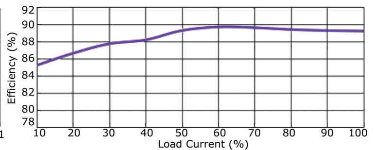
VX07815-500 Efficiency Curve Negative Output, Efficiency vs. Load Current (at Vin nominal)
