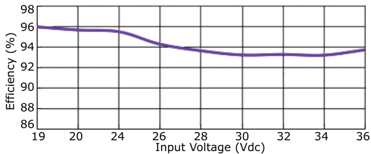
VX07815-500 Efficiency Curve Positive Output, Efficiency vs. Input Voltage (at full load)
