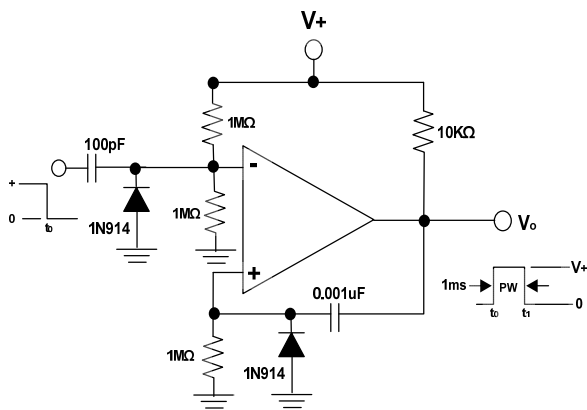
One-Shot Multivibrator
