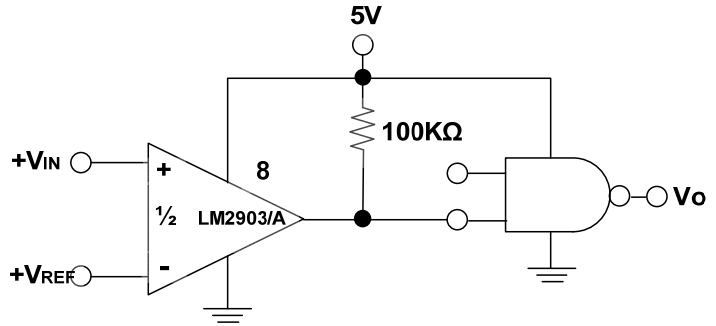
Driving CMOS
