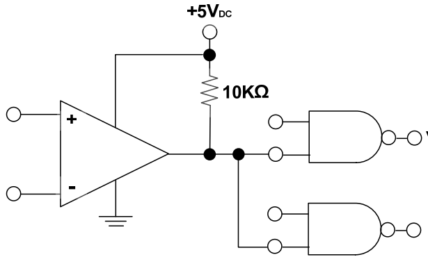
Driving TTL
