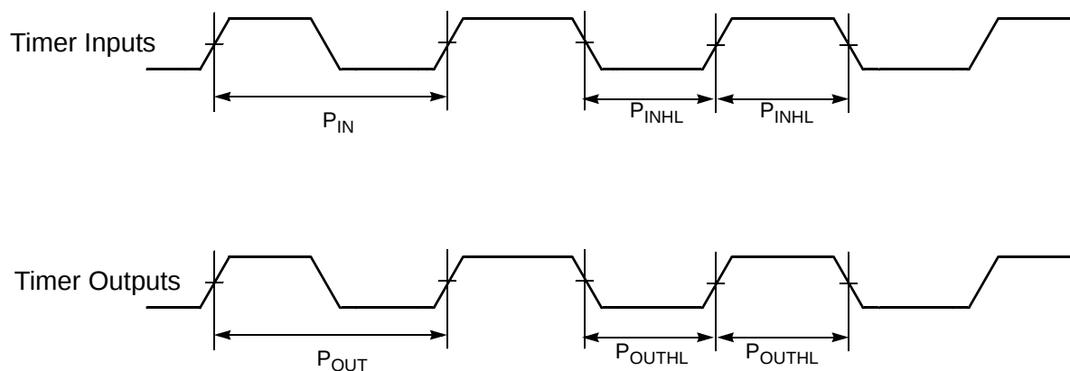
Figure 3-23 Timer Timing
