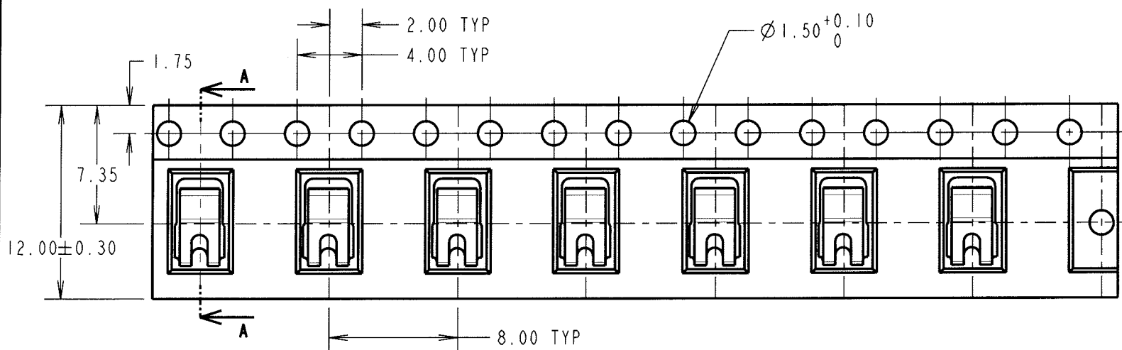
TAPE DIMENSIONS
