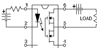
"B" Connection
