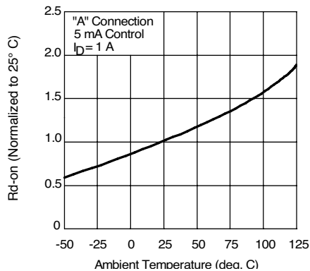
Figure 4. Typical Normalized On-Resistance
