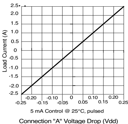
Figure 3. Linearity Characteristics
