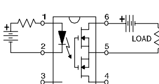
"B" Connection
