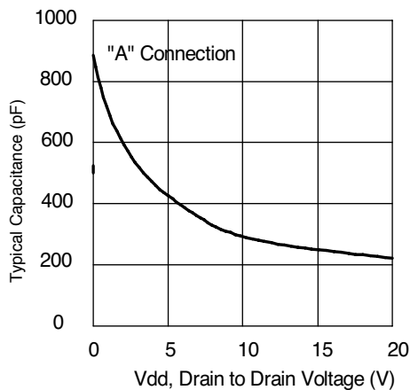
Figure 2. Typical Output Capacitance
