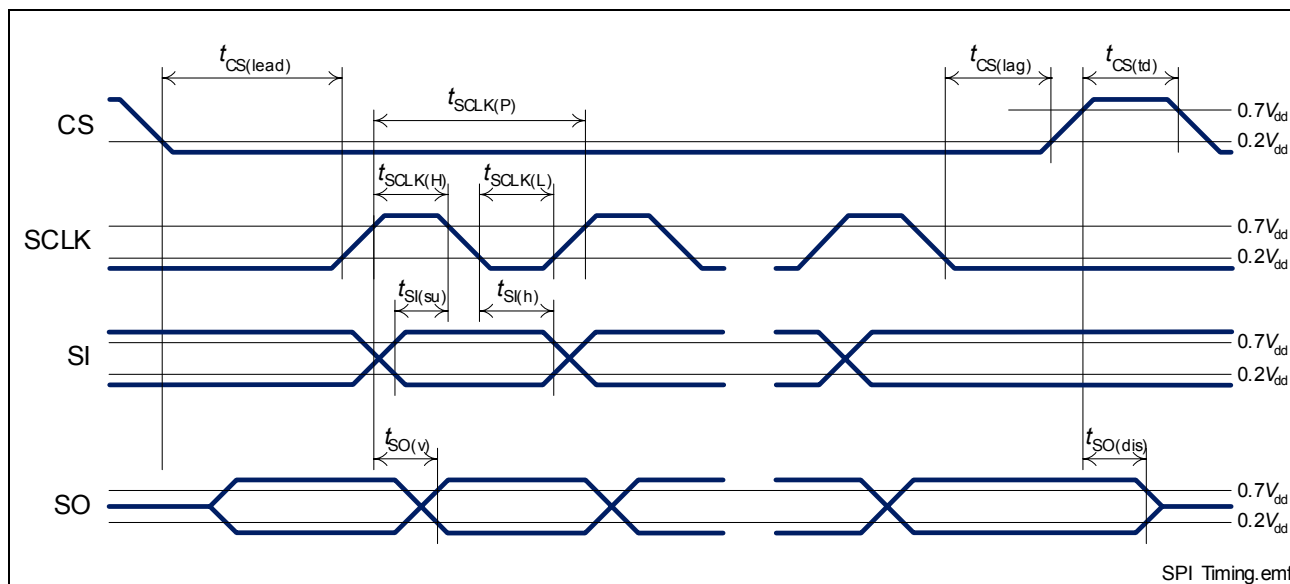
Figure 13 Timing Diagram
