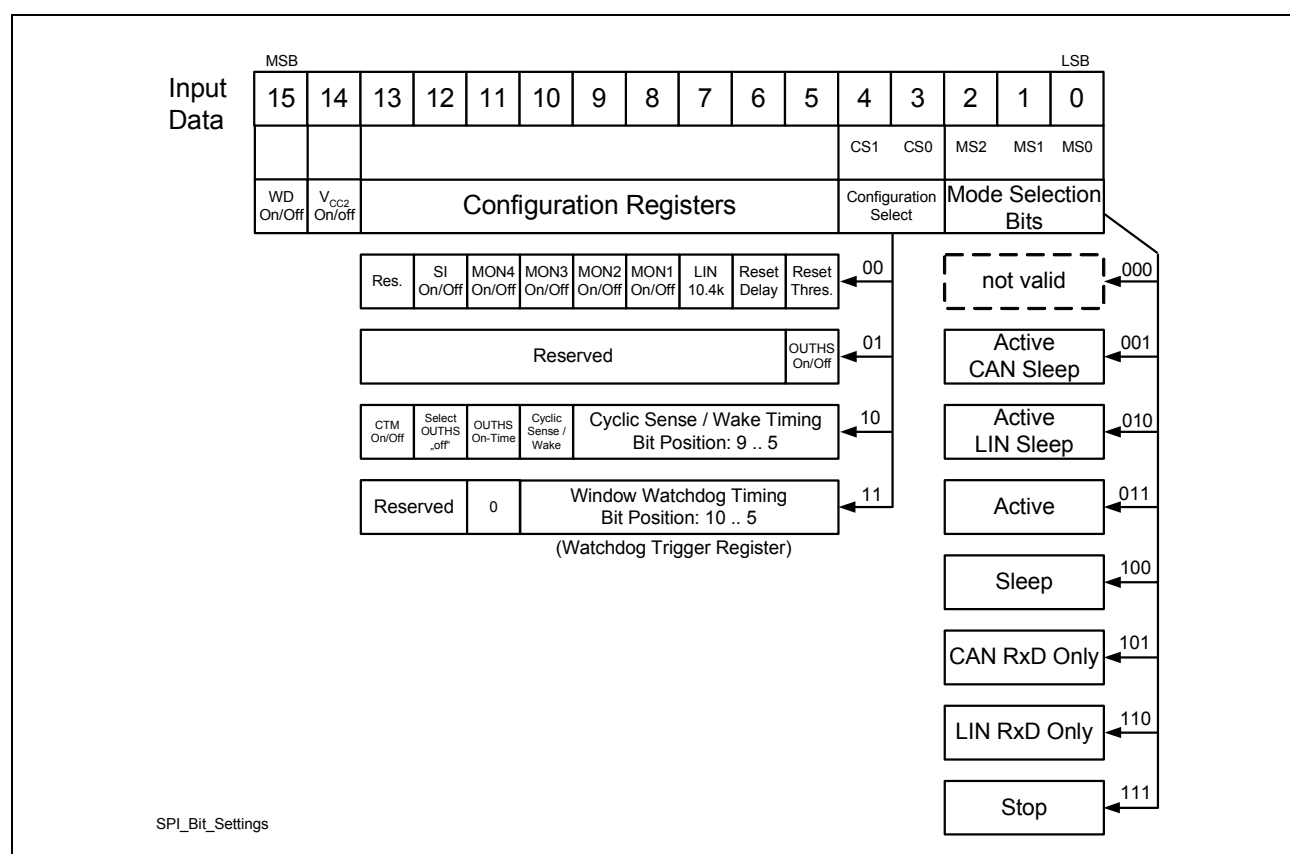
Figure 11 16-Bit SPI Input Data / Control Word
