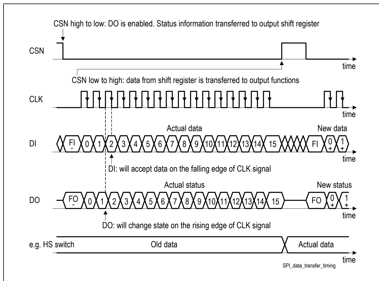
Figure 12 SPI-Data Transfer Timing
