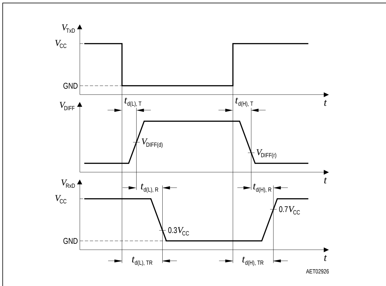
Figure 20 CAN Dynamic Characteristics Timing Diagram
