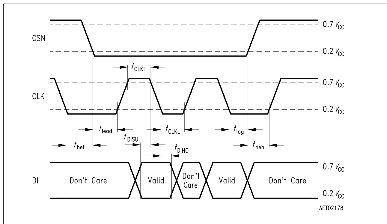
Figure 13 SPI-Input Timing
