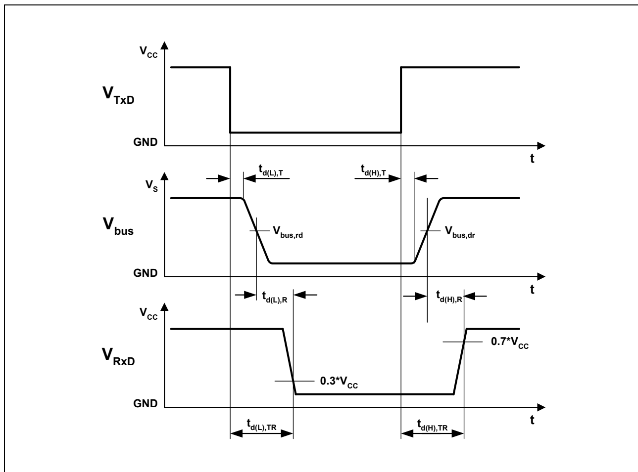
Figure 21 LIN Dynamic Characteristics Timing Diagram
