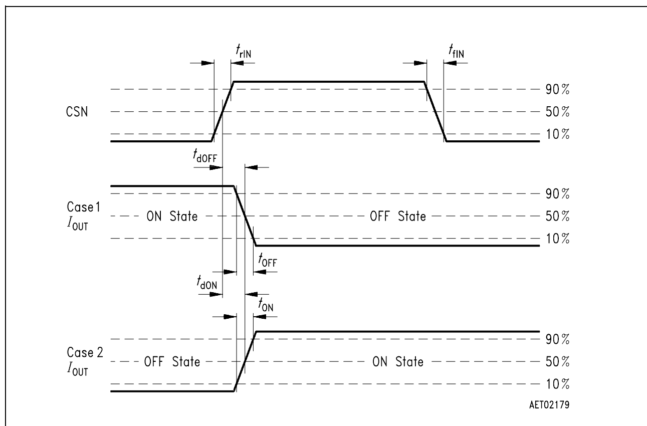
Figure 14 Turn OFF/ON Time
