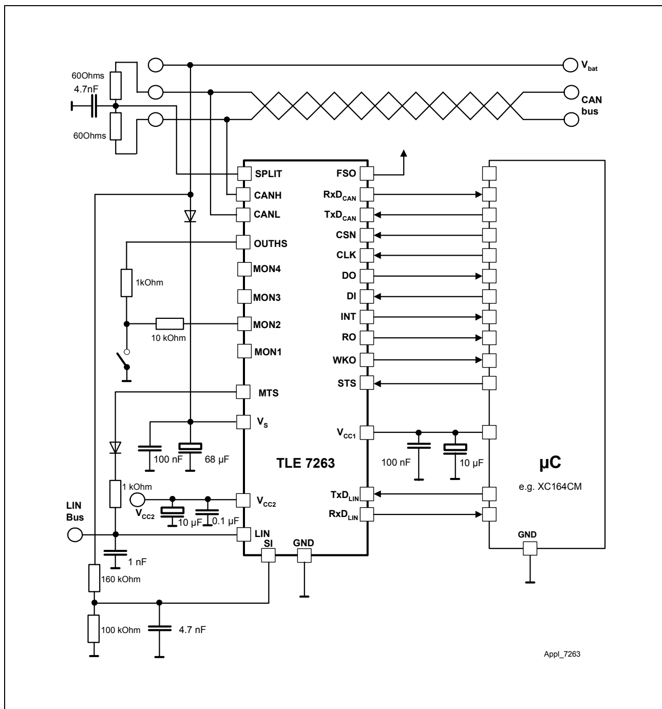
Figure 22 Application Circuit
