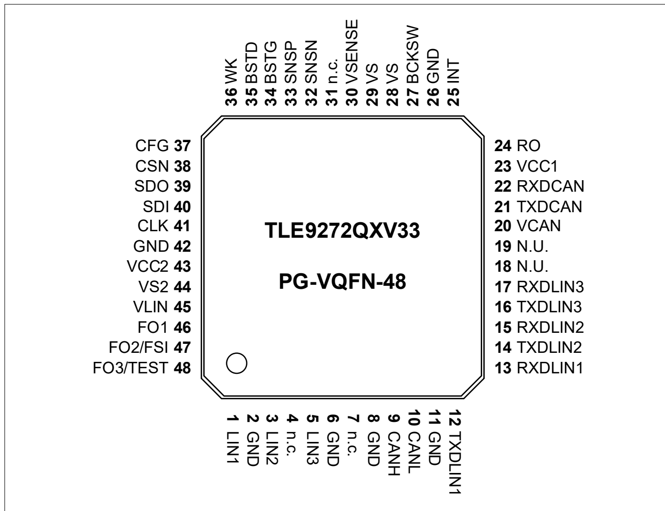
Figure 2 Pin Configuration
