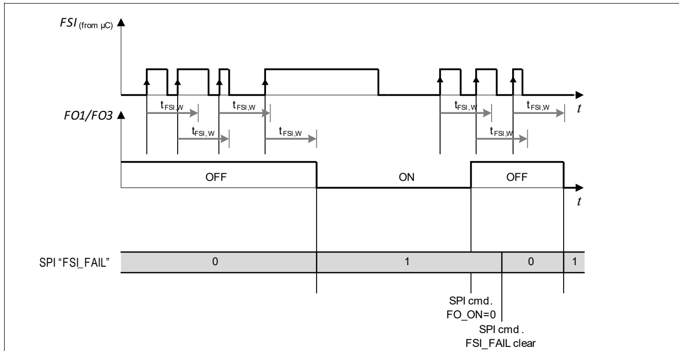
Figure 35 FSI timing diagram and level description
