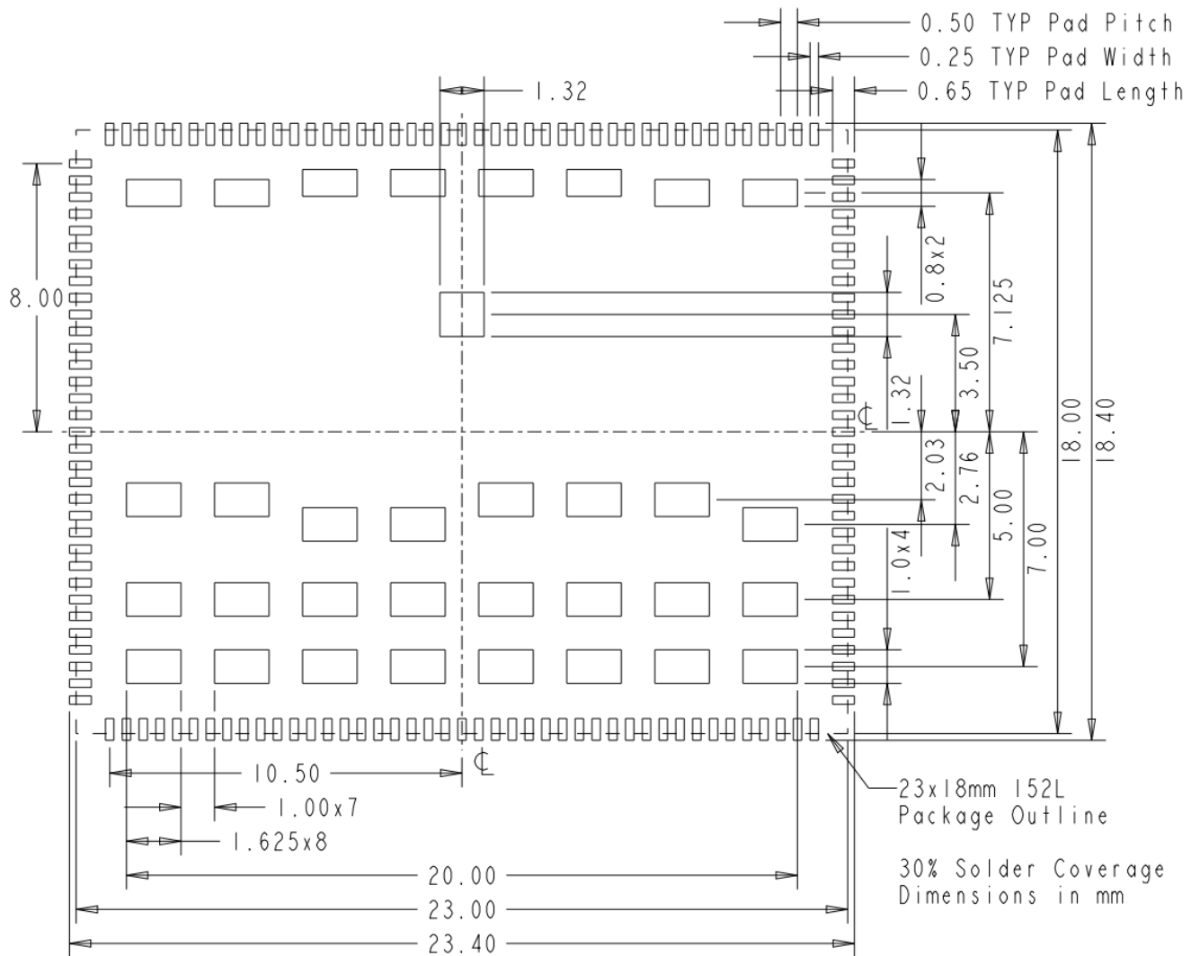
Figure 24: 30% Solder Stencil Aperture
