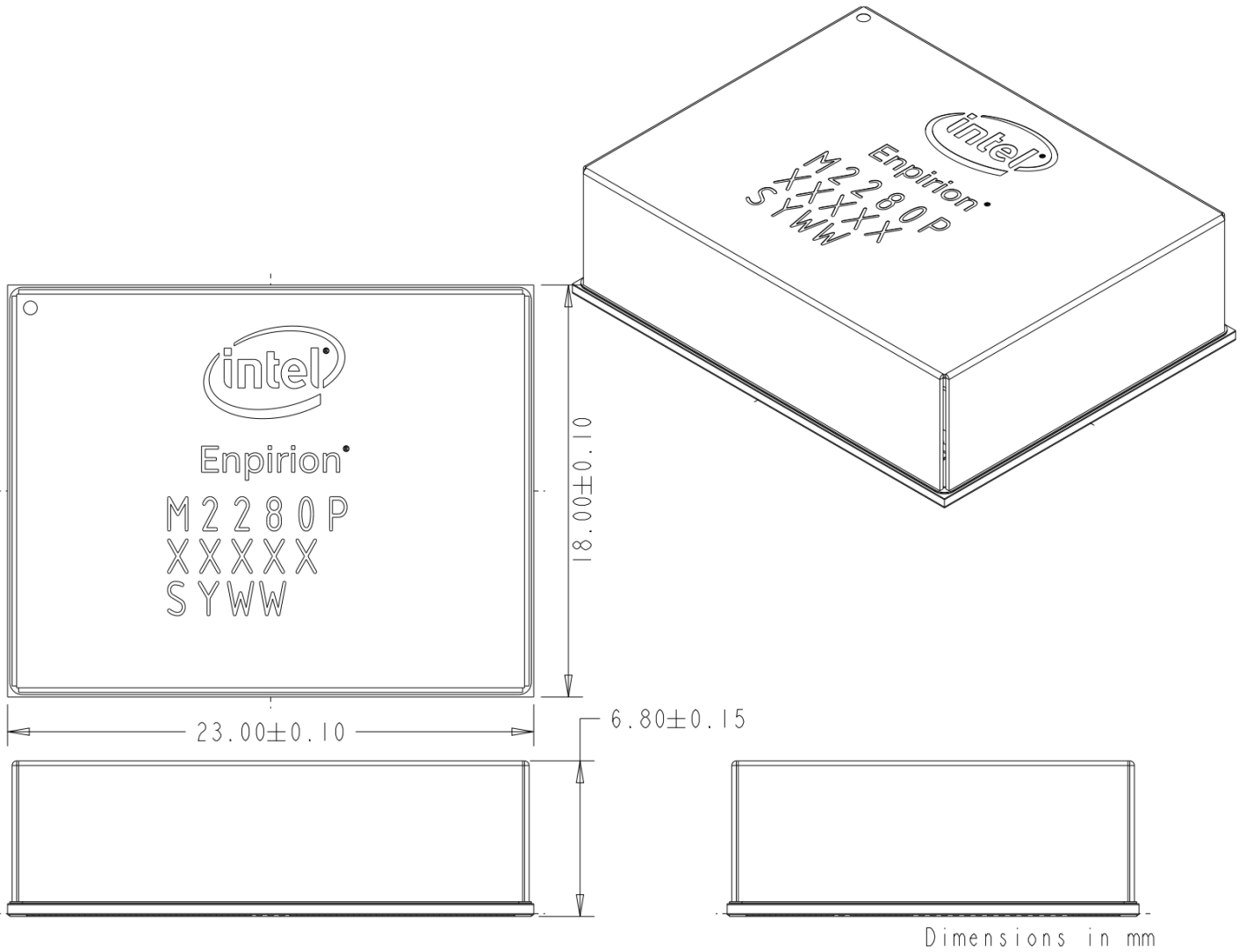
Figure 25: Package Dimensions 1/2
