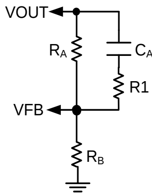
Figure 6: External Feedback/Compensation Network
