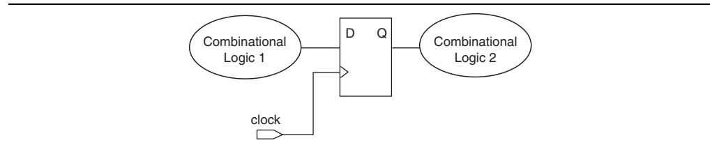
Figure 4. Registering Combinational Output Signal
