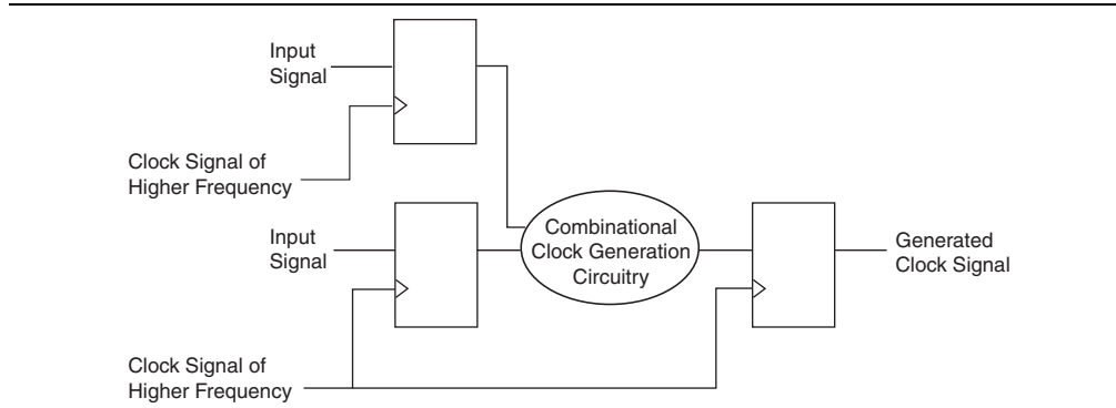
Figure 5. Registering the Input and Output Signals
