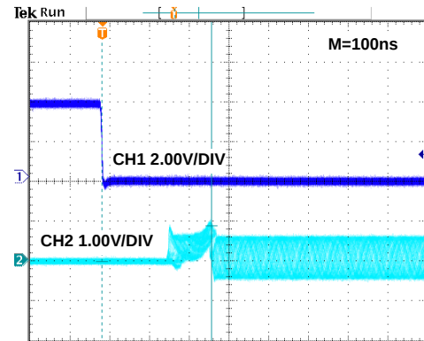
FIGURE 10. ENABLED RESPONSE
