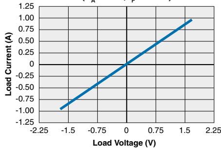
CPC1978 Typical Load Current vs. Load Voltage ( T_A = 25^\circ\text{C} , I_F = 10\text{mA} )
