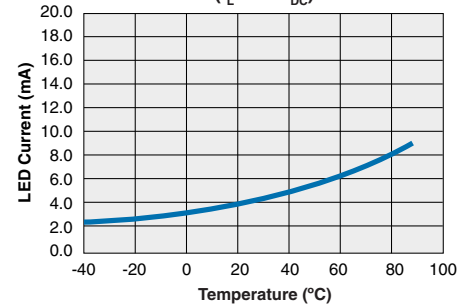
CPC1978 Typical I_F for Switch Operation vs. Temperature ( I_L = 0.5A_{DC} )
