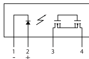
CPC1981Y Pinout
