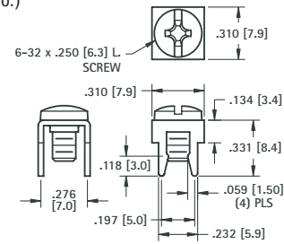
Mounting Detail
