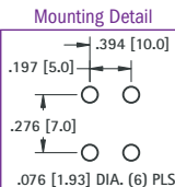
Mounting Detail
