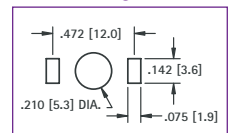
Mounting Detail
