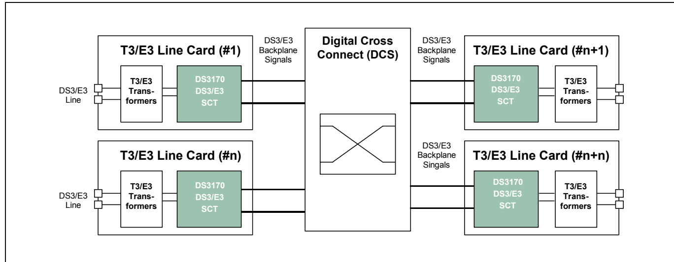
Figure 3-1. DS3/E3 Line Card
