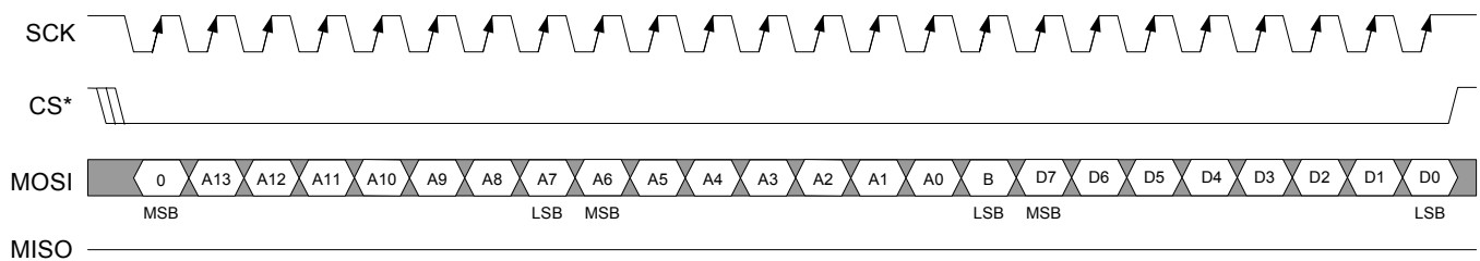
Figure 8-26. SPI Serial Port Access For Write Mode, SPI_CPOL = 1, SPI_CPHA = 1
