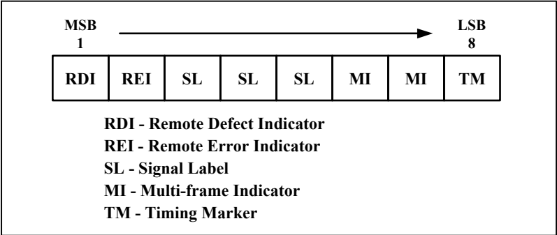
Figure 10-18. MA Byte Format
