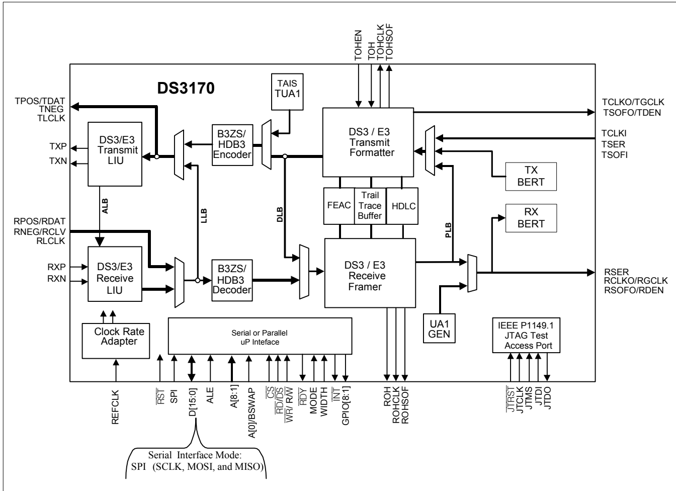
Figure 2-2. Block Diagram
