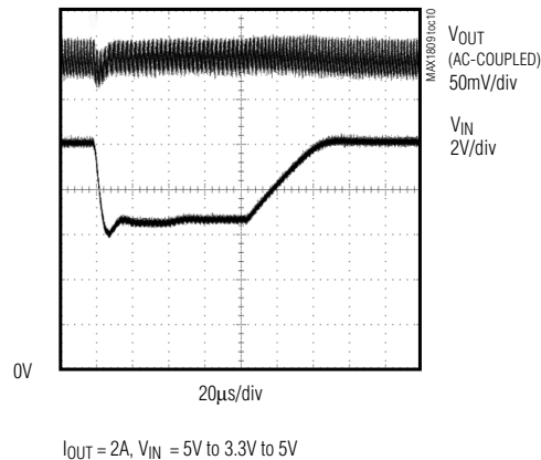
LINE-TRANSIENT RESPONSE
