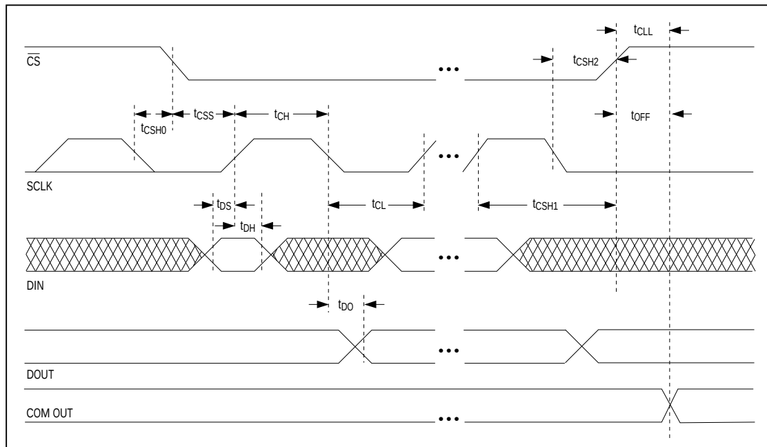
Figure 1. Timing Diagram
