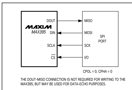
Figure 4. Connections for SPI and QSPI
