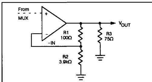
Figure 2. Unity-Gain Connections
