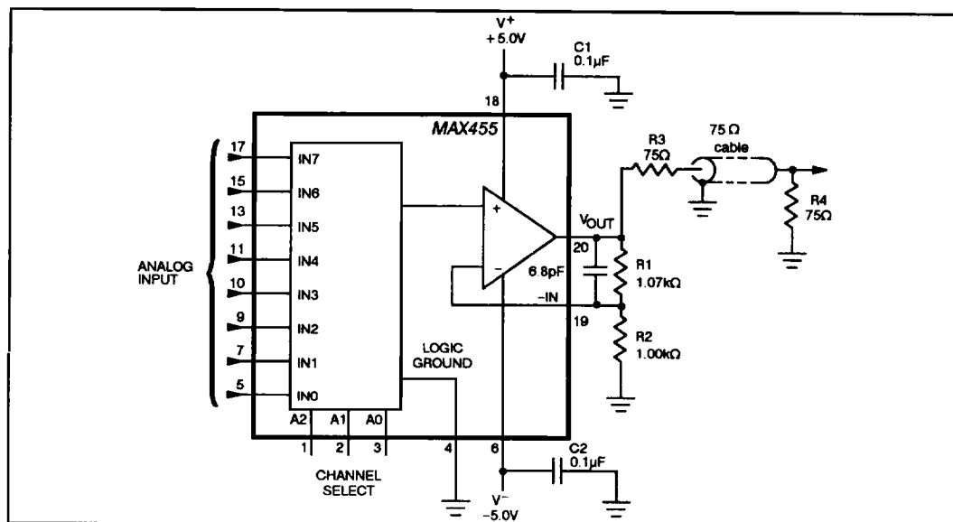
Figure 1. Typical Application
