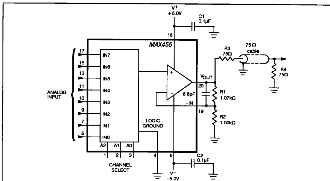
Figure 1. Typical Application
