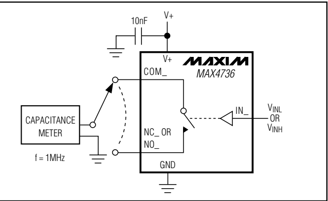
Figure 4. Channel Off/On-Capacitance
