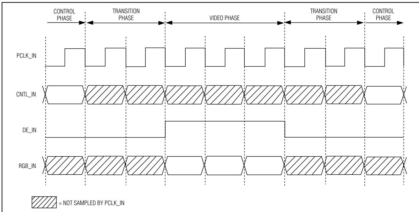
Figure 9. Transition Timing
