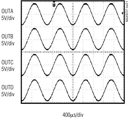
OUTPUT AT 2VRMS AT 1kHz ( V_{DD} = 5V , R_L = 1k\Omega )
