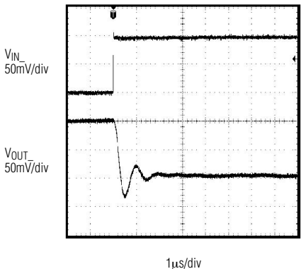
STEP RESPONSE
